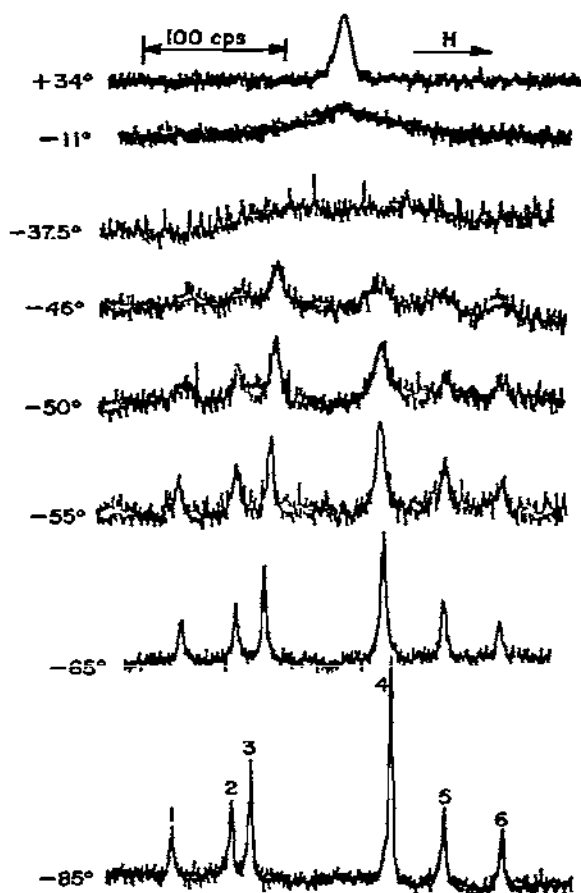
Fig. 26. The coalescence of the fluorine resonances of Ti(bzac)_2F_2 in dichloromethane (Ref 93, courtesy of Inorganic Chemistry).
