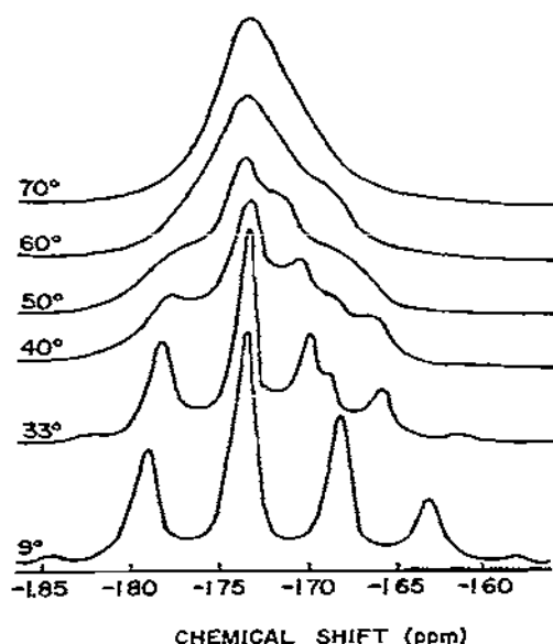
Fig 31. The coalescence of the methyl proton resonances for a Zr(tfa)_x(acac)_{4-x} ( x = 0 - 4 ) mixture in benzene. (Ref. 120, courtesy of Inorganic Chemistry).
