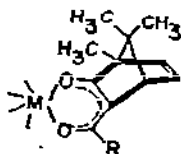
Fig. 20 An illustration of asymmetric d -camphorate ligands: 3-hydroxymethylene- d -camphorate if \text{R}=\text{H} , 3-acetyl- d -camphorate if \text{R}=\text{CH}_3 .
