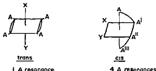
Fig. 22. The two geometrical isomers of an M(AA)_2XY complex illustrating the number of different resonances possible for the terminal groups of the AA ligands
