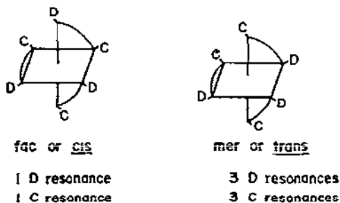
Fig. 17. The two geometrical isomers of an M(CD)_3 complex illustrating the number of different resonances possible for each terminal group
