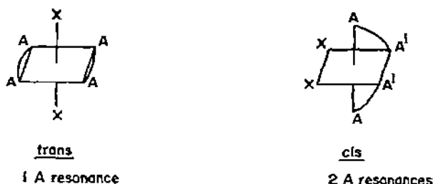
Fig. 21. The two geometrical isomers of an M(AA)_2X_2 complex illustrating the number of different resonances possible for the terminal groups of the AA ligands.
