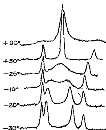
Fig. 29 The coalescence of the fluorine resonances of (\pi\text{-C}_5\text{H}_5)\text{Zr}(\text{hfa})_3 in methylcyclohexane at 50 - 90^\circ\text{C} and acetone at the lower temperatures. The spectra of the complex have been aligned vertically although the chemical shifts differ appreciably in the two solvents (Ref 109, courtesy of the Journal of the American Chemical Society)
